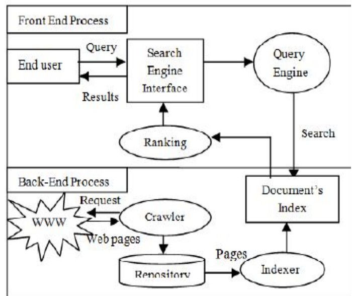
Fig. 1 Architecture of search engine
