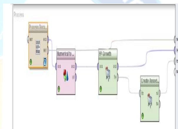
Fig. 3. Transformation and processing of data in RapidMiner
