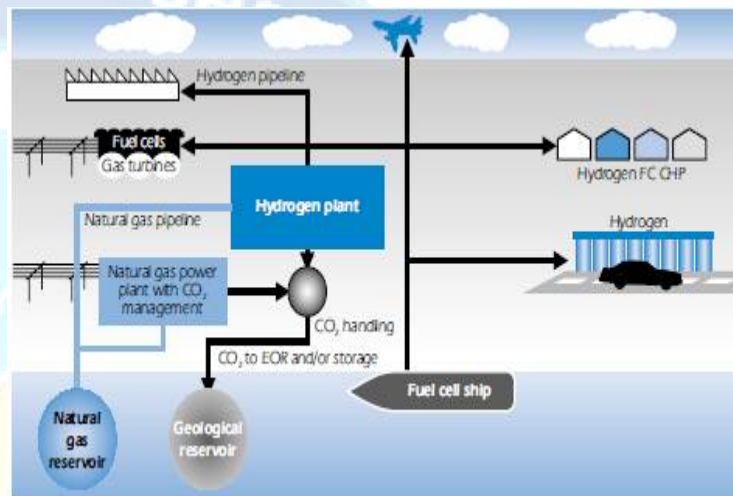
Fig. 1. Centralized hydrogen Production
