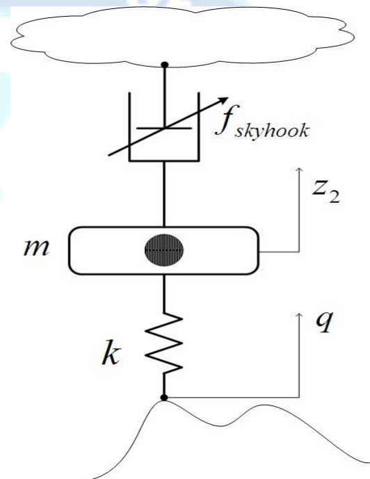
Fig 1: Ideal Skyhook control scheme.
