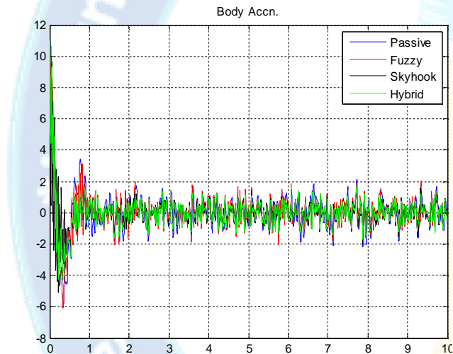
Fig 7: Combined Plot of Body Accn.
