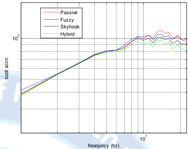
Fig 9: Transformation Function of Body Acceleration (Enlarge View).
