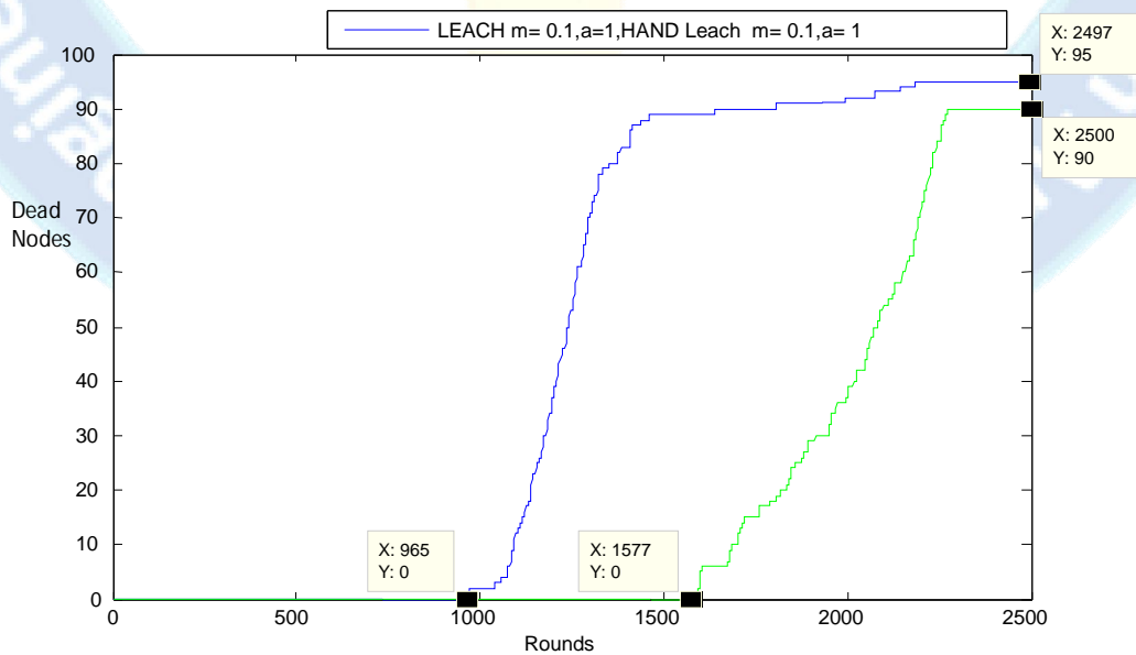
Fig 3(b). No. of dead nodes at different rounds.
