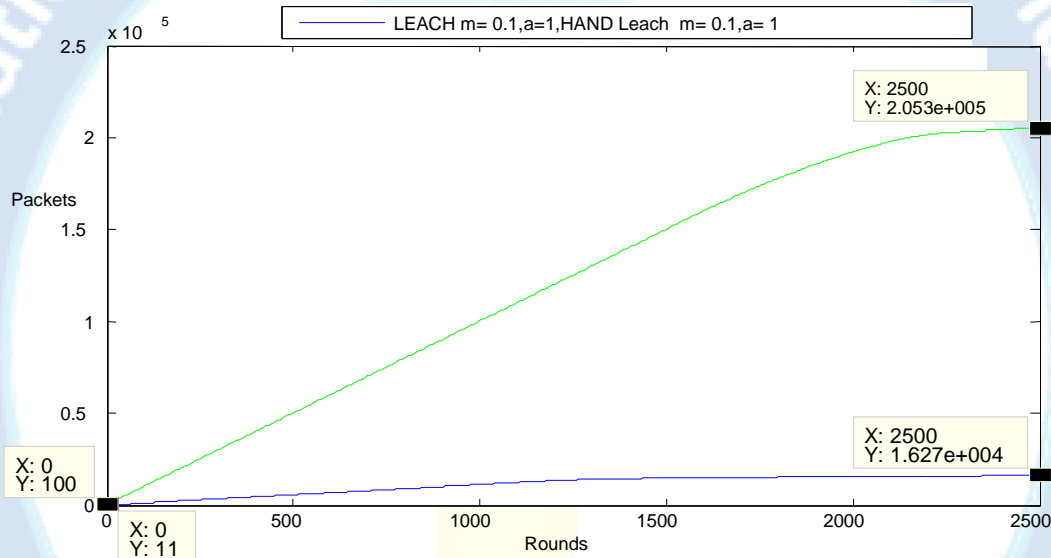
Fig 3(a). Number of Packets Sent at different rounds.
